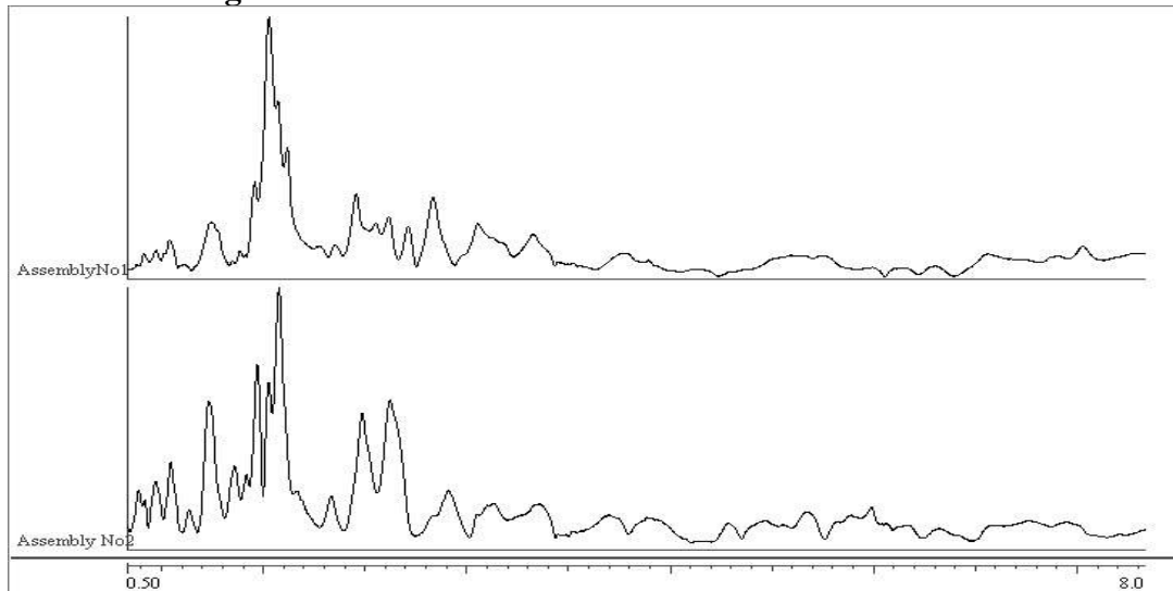
Figure 4. Waveforms for Identical Bracket Assemblies
