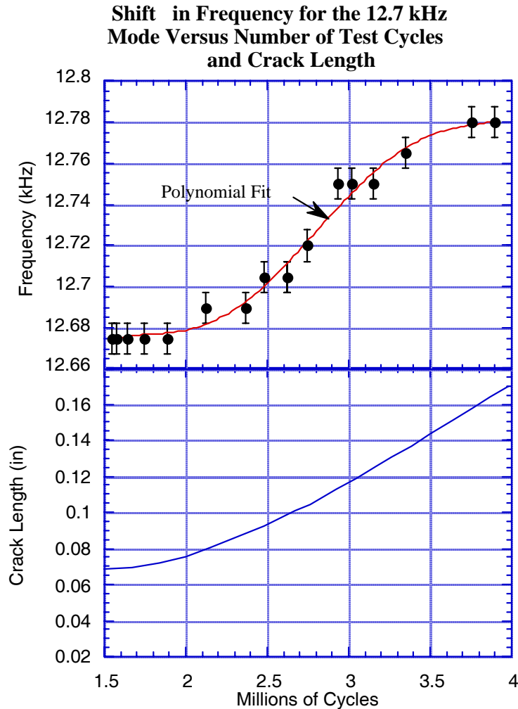
Figure 7. Frequency Shift vs. Crack Length
