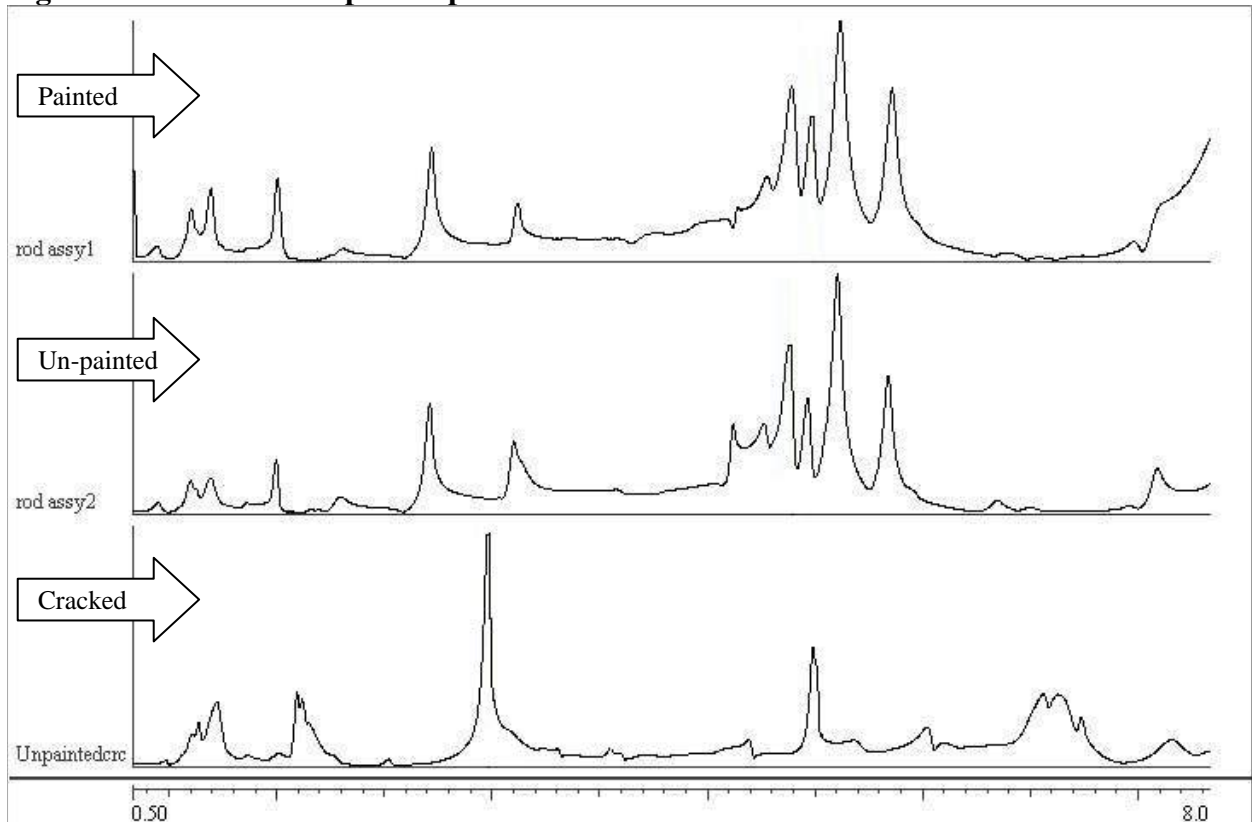
Figure 2. Waveform Output - Input Rod Assemblies
