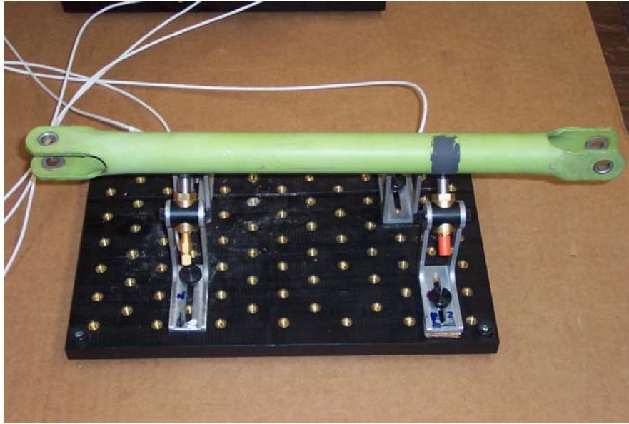
Figure 1. Input Rod Assembly
