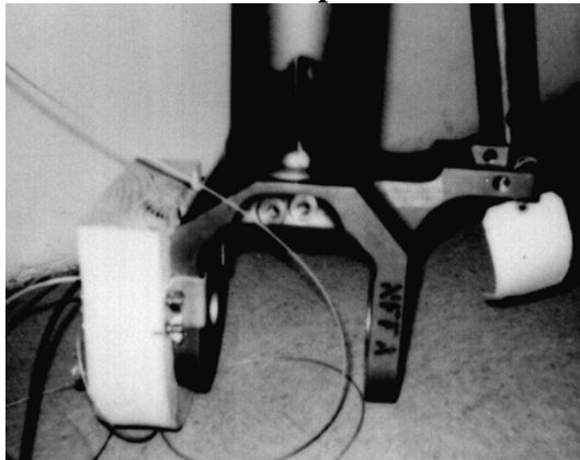
Figure 5. Helicopter Spindle Test Setup
